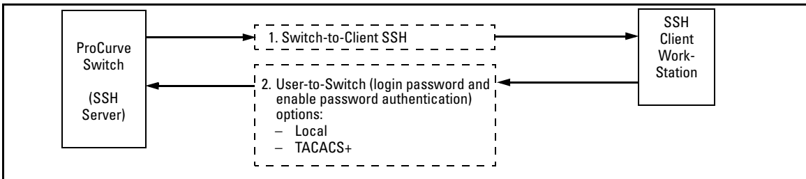
Figure 7-2. Switch/User Authentication
